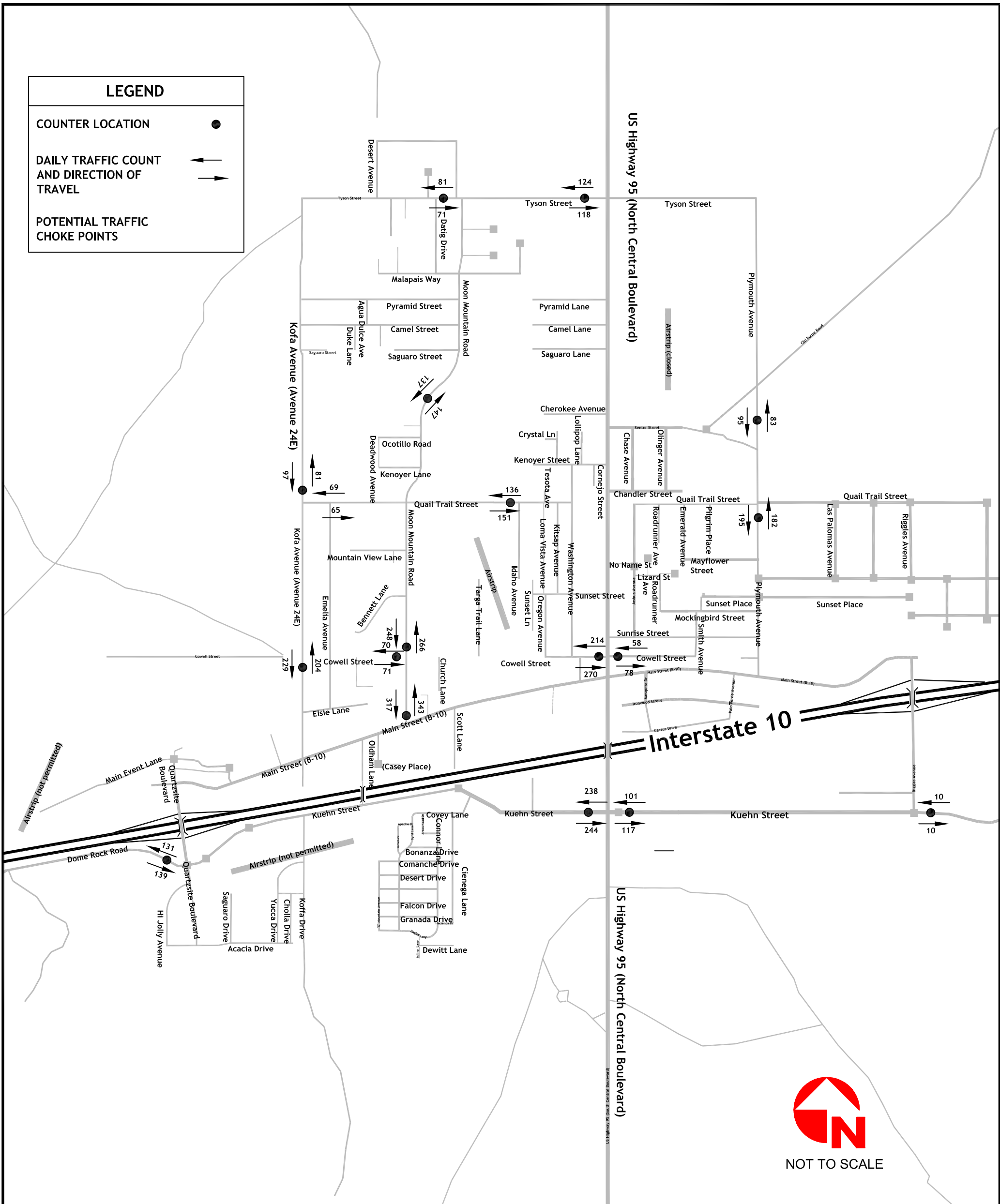
EXHIBIT T-7 TRAFFIC COUNTS AUGUST 2002
